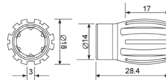
CX-JS Dimensions (mm)
