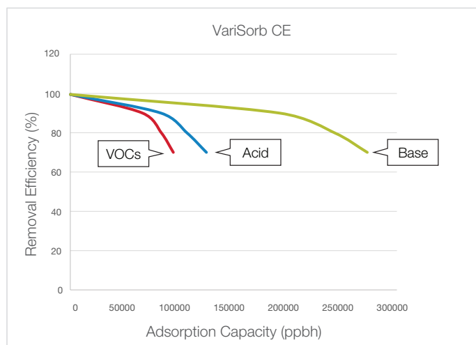
Removal Efficiency Curve
