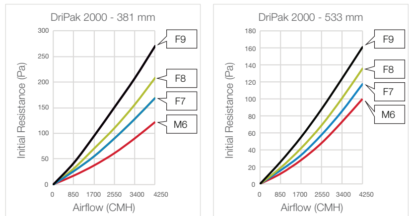
Initial Resistance vs. Airflow
