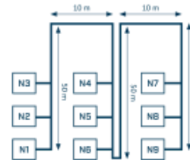
Conventional bus structure The distance between the two nodes furthest apart (1/9) is 220 meters.
