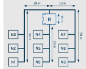
Extended structure with drop line The distance between the two nodes furthest apart (1/6 or 6/9) is 145 meters.
