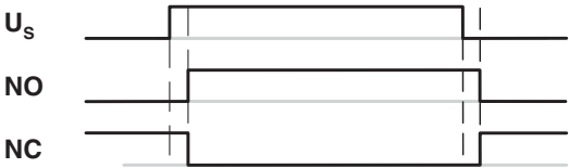
Figure 1 Time diagram for automatic start
