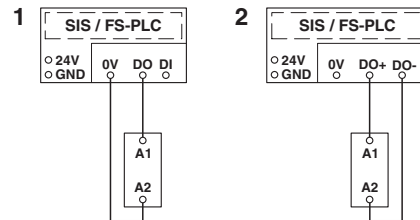
Figure 8 Signal generator connection versions
