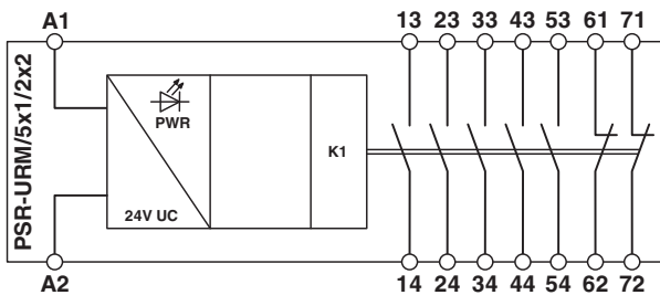
Figure 2 Block diagram
