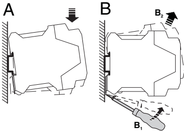
Figure 5 Mounting and removing
