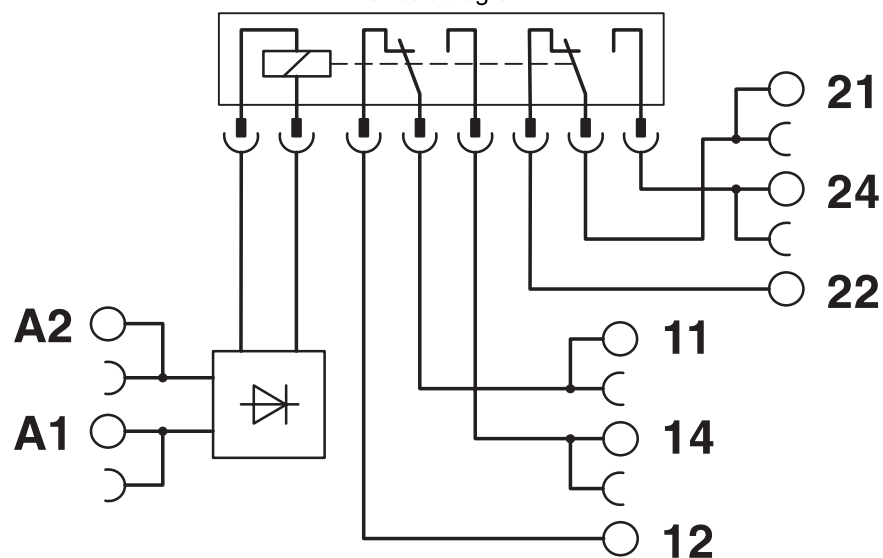
Circuit diagram
