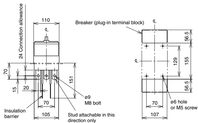
Drilling plan
