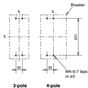
Drilling plan
