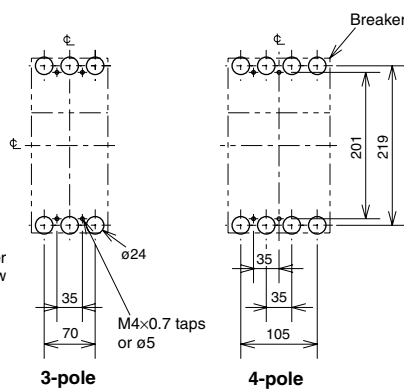
Drilling plan
