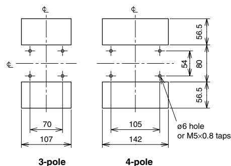
Drilling plan
