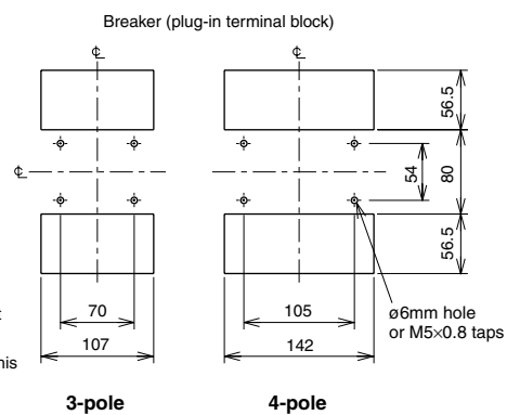
Drilling plan
