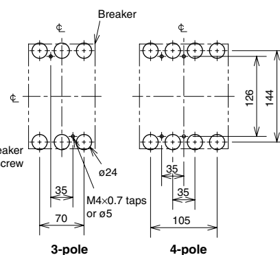
Drilling plan
