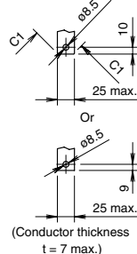
Conductor drilling for direct connection
