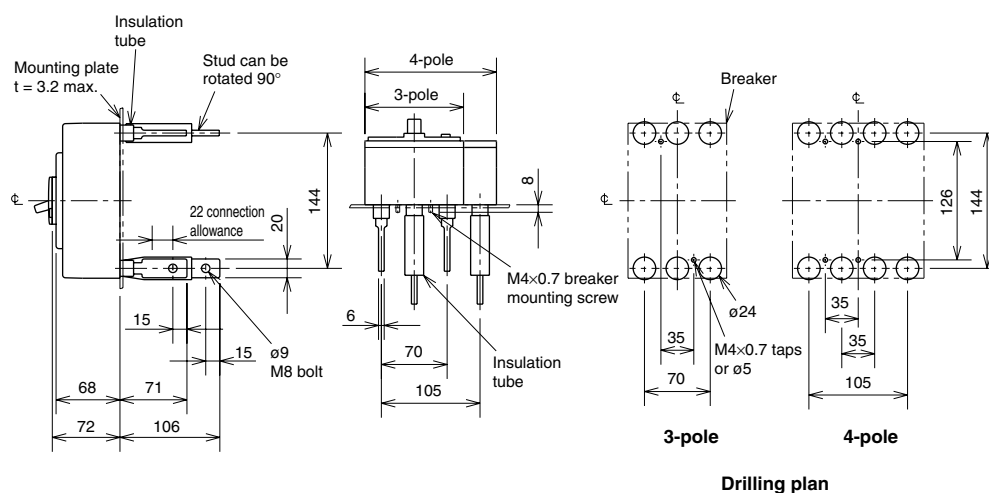
Drilling plan
