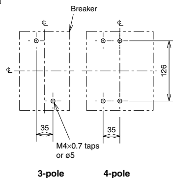
Drilling plan
