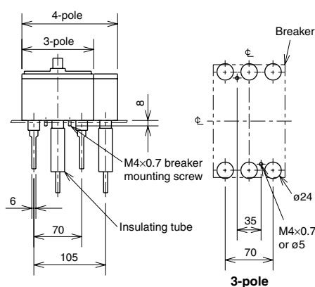
Drilling plan
