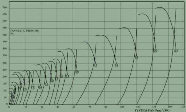
Volume Flow M3/h x 1000
