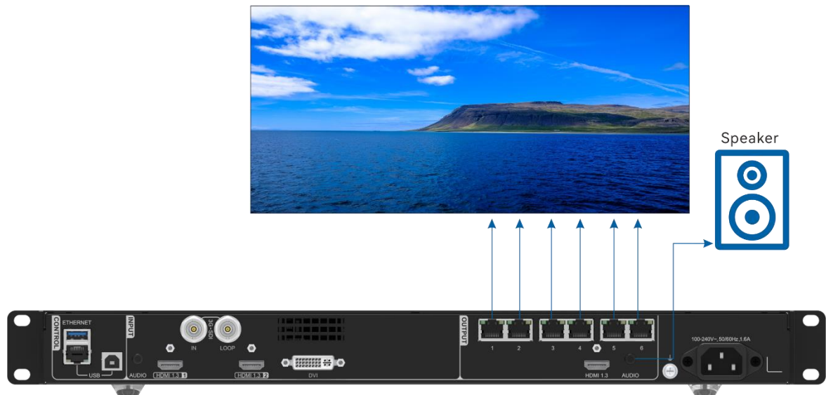
Figure 5-39 Audio output connection-2
