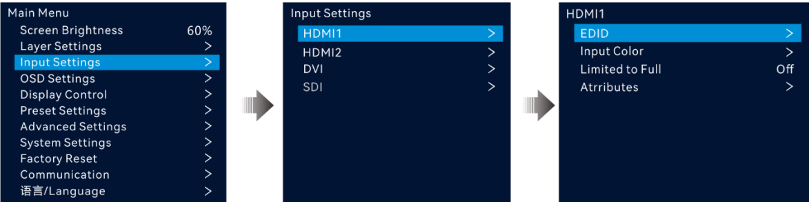
Figure 5-8 Input source selection
