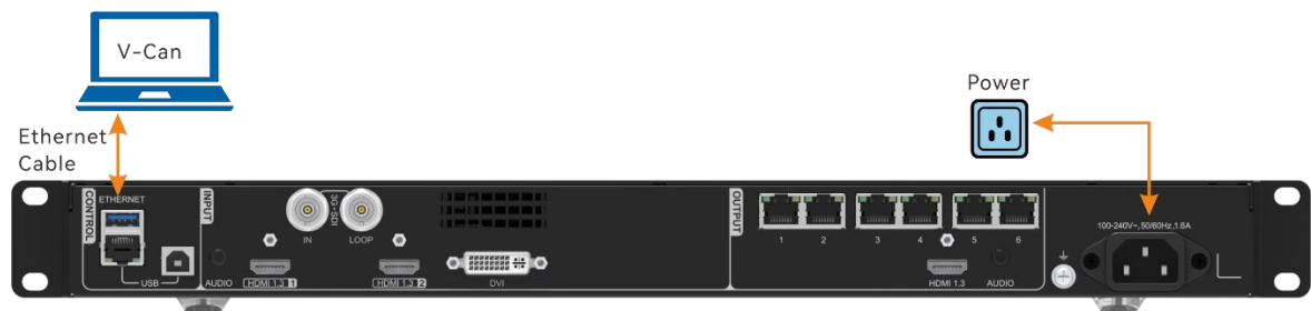
Figure 6-1 Hardware connection
