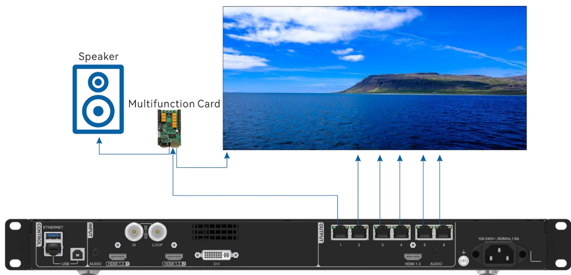
Figure 5-38 Audio output connection-1
