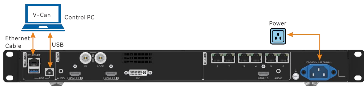
Figure 5-12 Hardware connection
