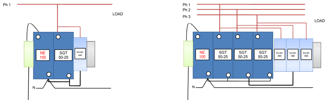
Figure 1 - Connection and Wiring Method (Kelvin Method) for 1Ph and 3Ph
