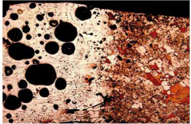
Hydrogen embrittlement in TIG welded, ETP
