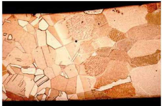
TIG welding seam in oxygen-free OF-OK® copper
